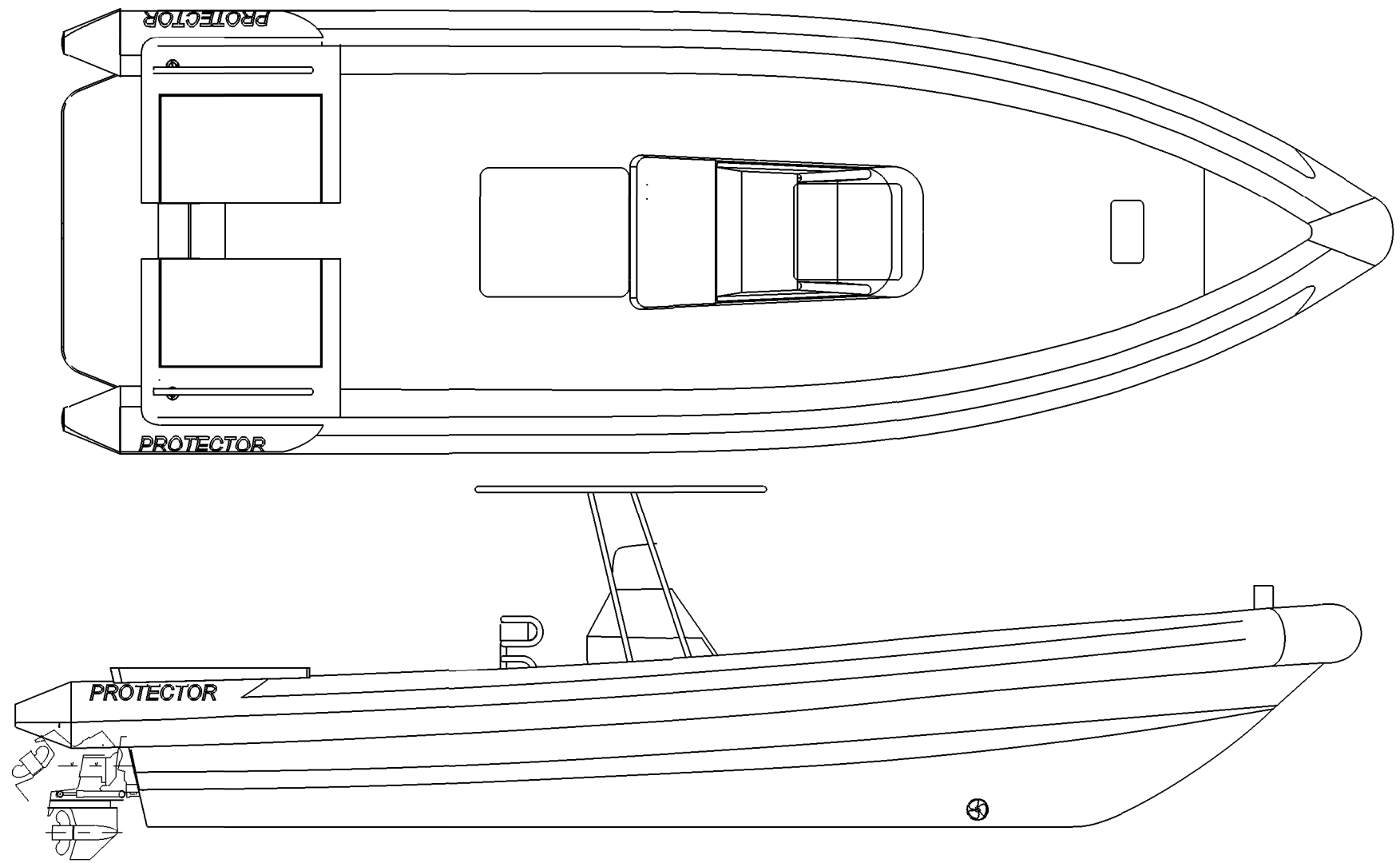
Protector 10.5mtr Centre Console Twin Inboard
